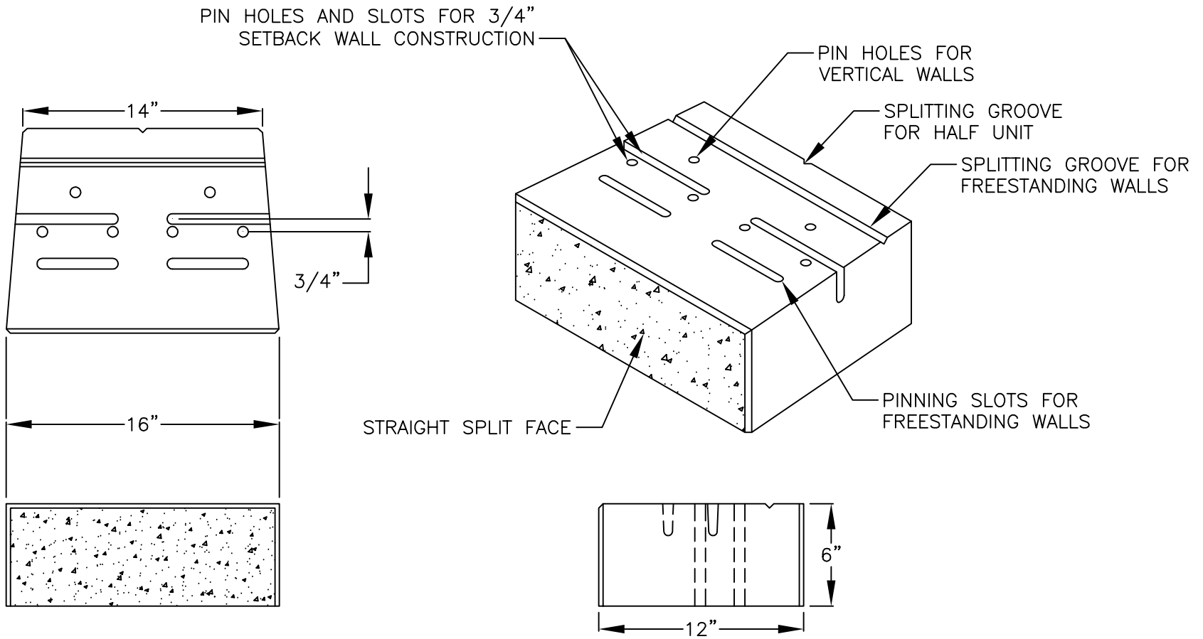
VERSA-LOK UNIT UNIT DIMENSIONS SCALE: NONE
